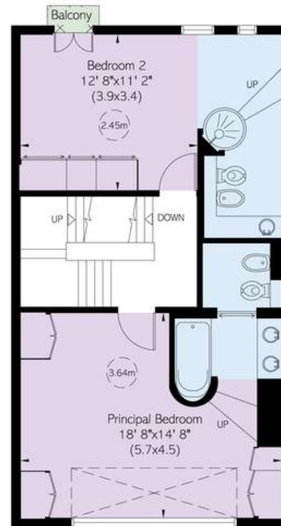
Second Floor
