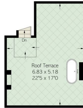
Third Floor
