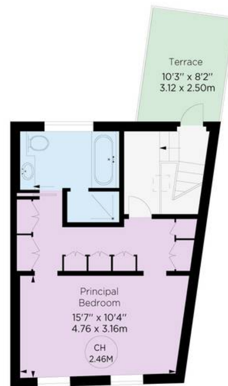
SECOND FLOOR
