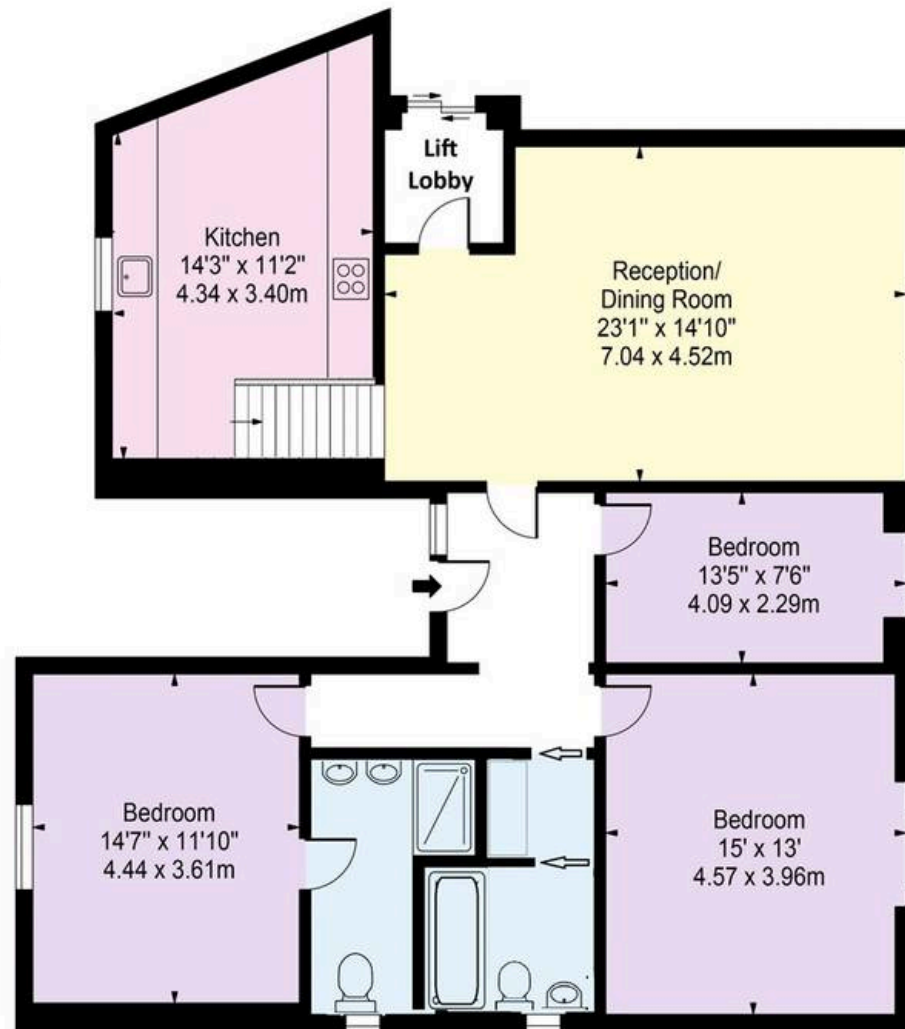
FIRST FLOOR
