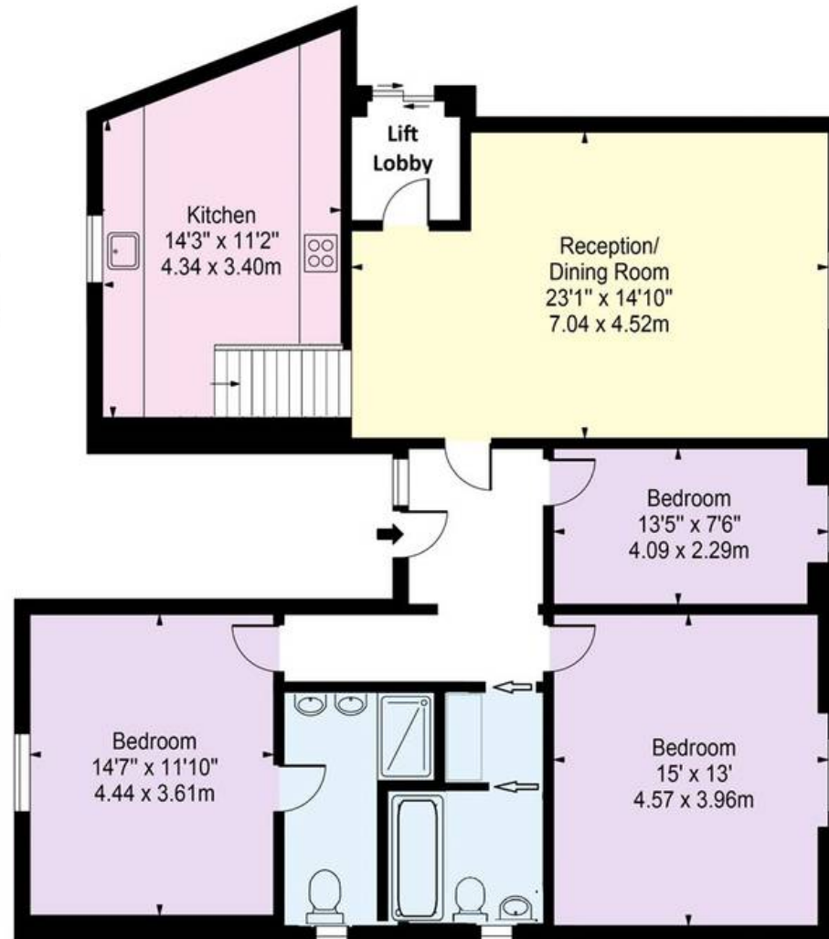
FIRST FLOOR
